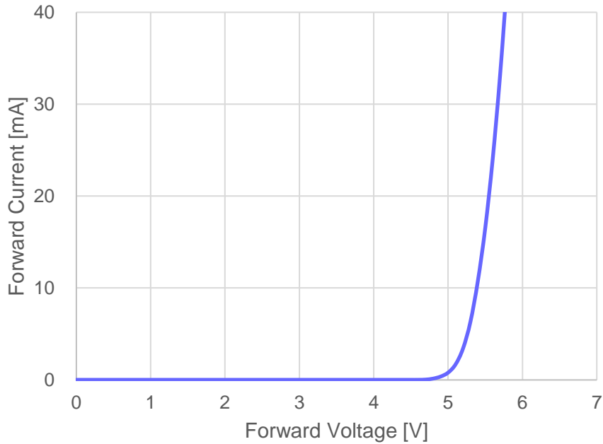
< Forward Voltage vs. Forward Current >
