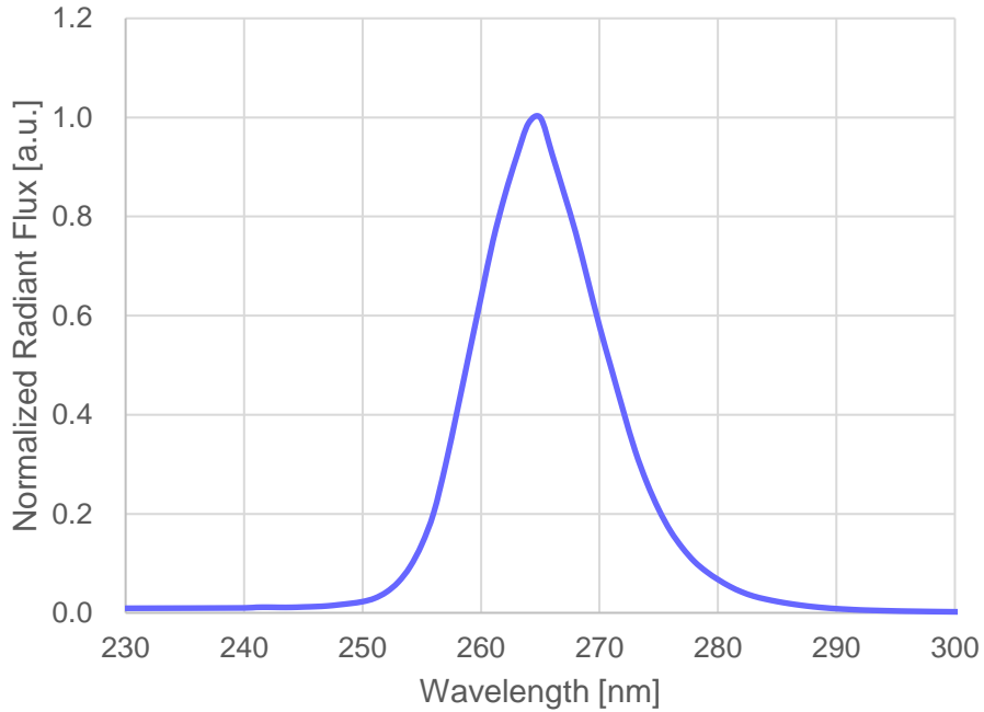
< Spectrum, I_F = 20\text{ mA} >
