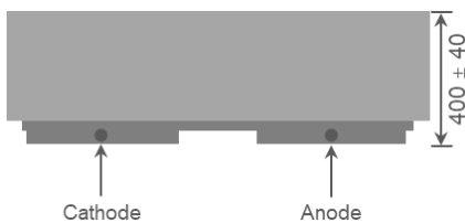
Cross Section
