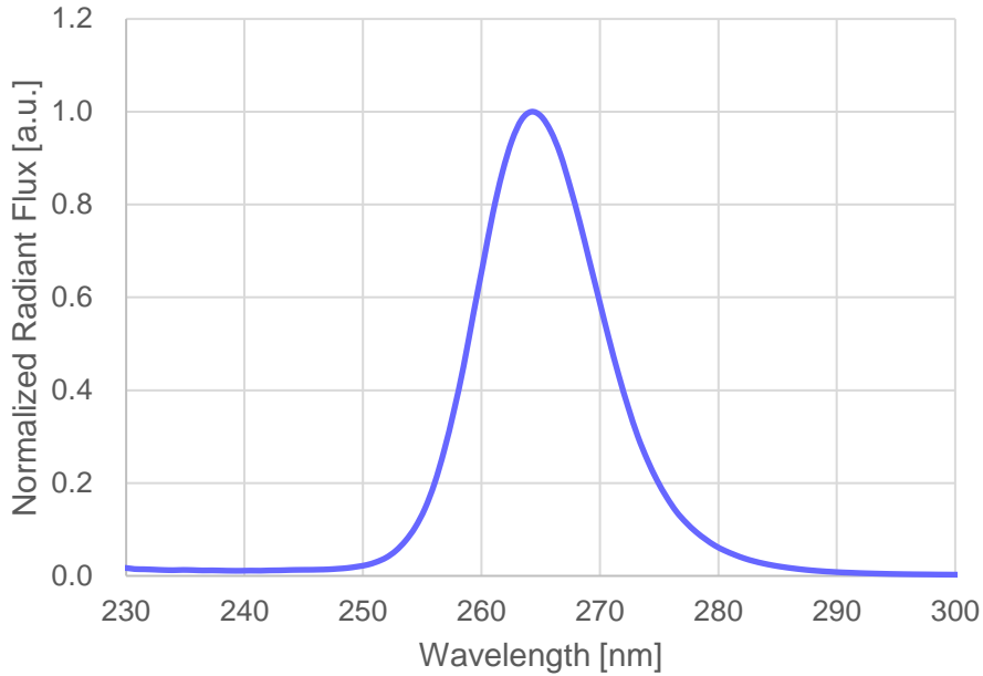
< Spectrum, I_F = 500\text{ mA} >
