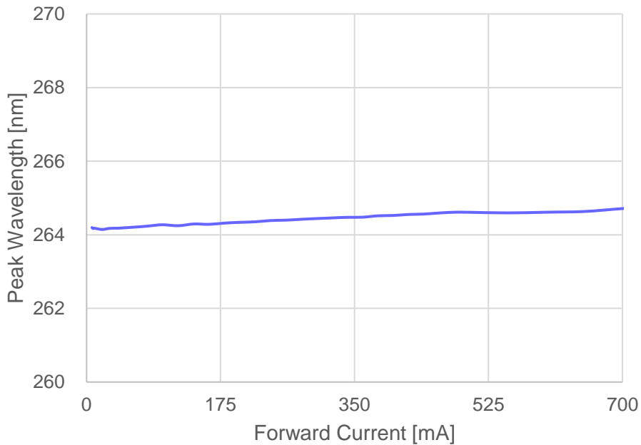
< Forward Current vs. Peak Wavelength >
