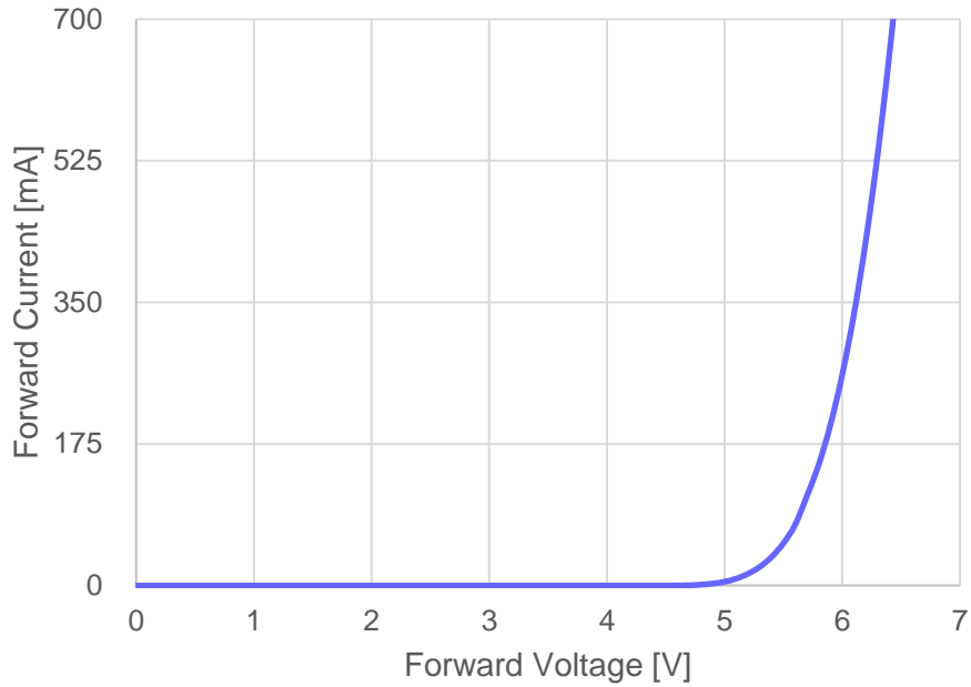
< Forward Voltage vs. Forward Current >
