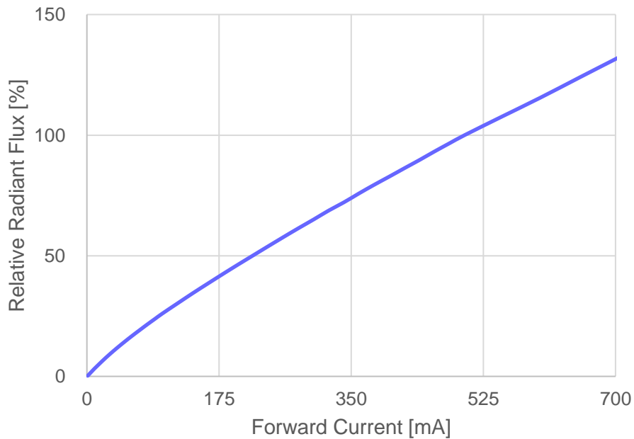
< Forward Current vs. Relative Radiant Flux >
